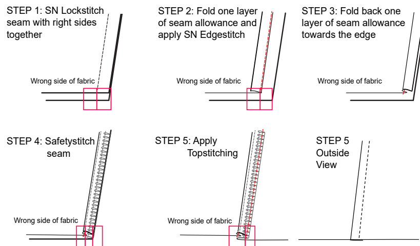
IMAGE 4.3: WOVEN HALF PINCH SEAMING
