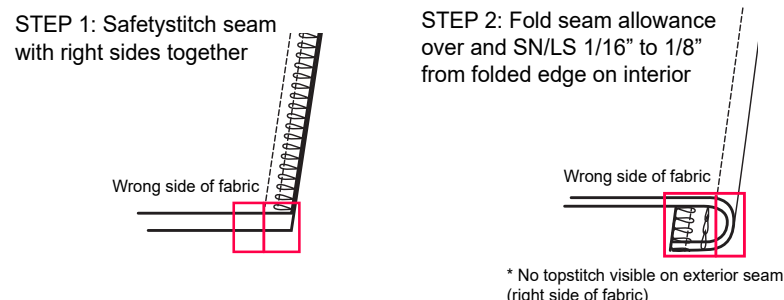
IMAGE 4.3: WOVEN HALF PINCH SEAMING
