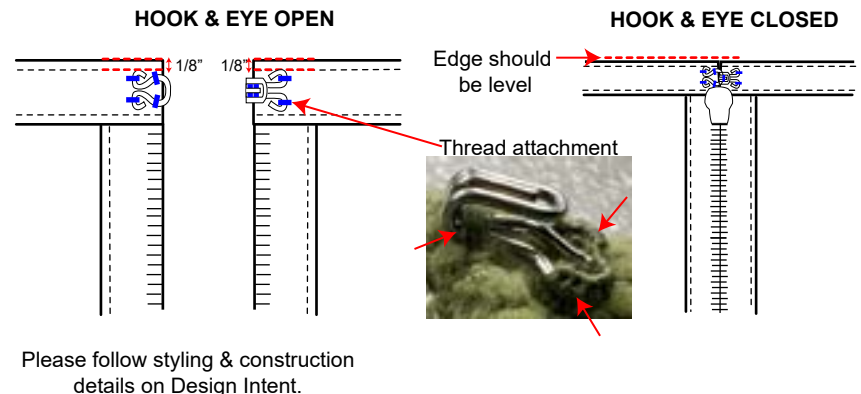
IMAGE 23: HOOK & EYE PLACEMENT
