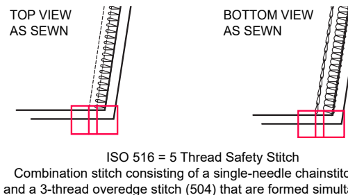
IMAGE 4.2: WOVEN PINCH SEAMING
