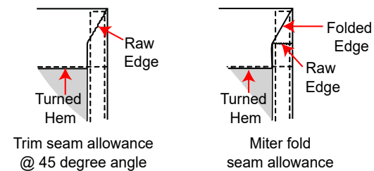
INNER CORNER POCKET TREATMENT
