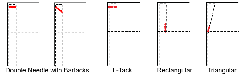
INNER CORNER POCKET TREATMENT
