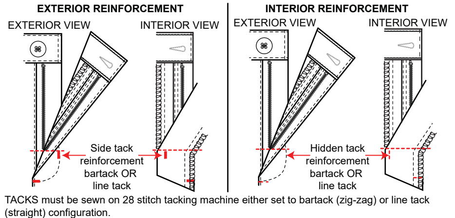
IMAGE 15: FLY SIDE TACK REINFORCEMENT
