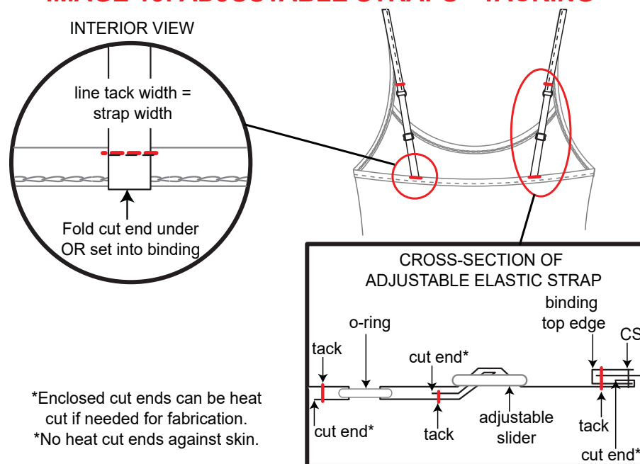
IMAGE 13: ADJUSTABLE STRAPS - TACKING
