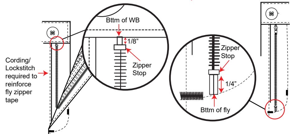
IMAGE 16: FLY - CORD STITCH, ZIPPER GAP
