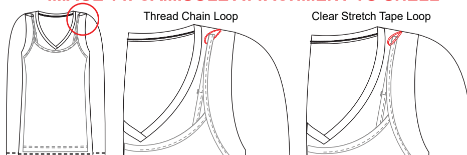
IMAGE 14: CAMISOLE ATTACHMENT TO SHELL
